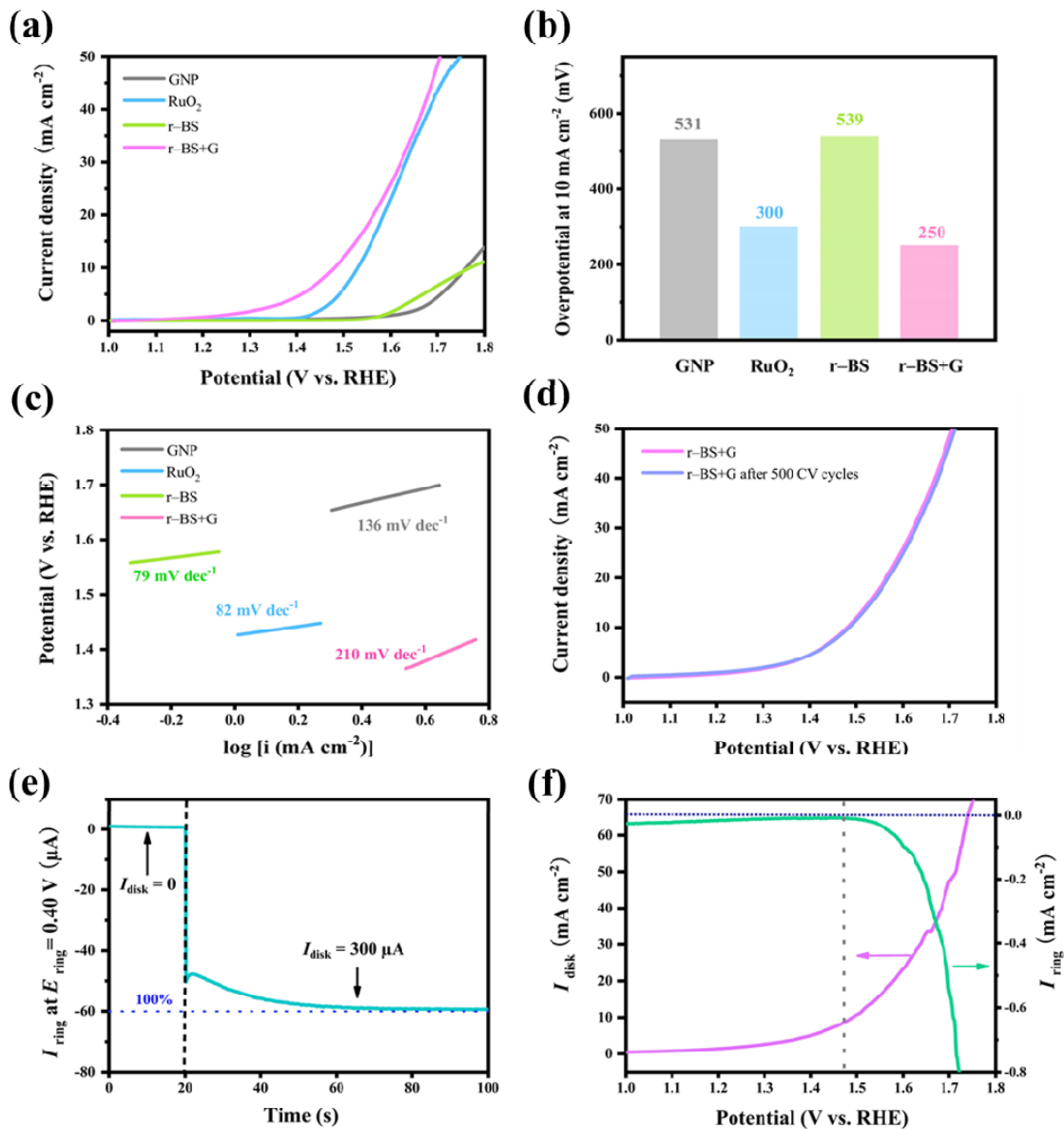
図 3 OER performances of various electrocatalysts. (a) LSV curves for the OER, (b) overpotentials at 10 \text{ mA cm}^{-2} , and (c) Tafel plots of various electrocatalysts. (d) LSV curves of r-BS+G recorded before and after 500 CV cycles between 1.20 and 1.53 V. (e) Faraday efficiency testing of r-BS+G using the rotating ring-disc electrode (RRDE) technique in Ar-saturated 1 M KOH solution. The ring current ( I_{\text{ring}} ) was measured at the potential of ring ( E_{\text{ring}} ) of 0.40 V vs. RHE, meanwhile the disc current ( I_{\text{disk}} ) is switched from 0 to 300 \mu\text{A} . The vertical dashed black line points to the time at which a 300 \mu\text{A} current was applied to the disc electrode, while the horizontal dashed blue line corresponds to the calculated 100% efficiency (60 \mu\text{A} ). (f) I_{\text{disk}} at the r-BS+G/glassy carbon disc electrode in Ar-saturated 1 M KOH (pink) and Pt ring (held at 0.2 V vs. RHE) current due to the ORR (green) as functions of the disc potential. The vertical dashed grey line shows the onset of the ORR at the ring electrode.
