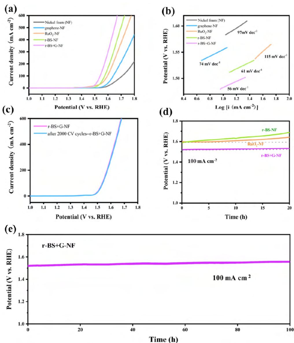
図 4 OER performance of various electrode catalysts. (a) LSV curve of OER, (b) Tafel plot, and (c) LSV curve of r-BS+G-NF taken before and after 2000 CV cycles between 1.20 and 1.53\text{ V} . (d, e) Change in potential when holding 100\text{ mA cm}^{-2} .
