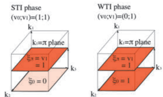
図3 強いトポロジカル絶縁体と弱いトポロジカル絶縁体(H.Araki, T. Kariyado, Y. Hatsugai "Entanglement Chern number for three-dimensional topological insulators: Characterization by Weyl points of entanglement Hamiltonians", Phys. Rev. B96, 165139 (2018))
